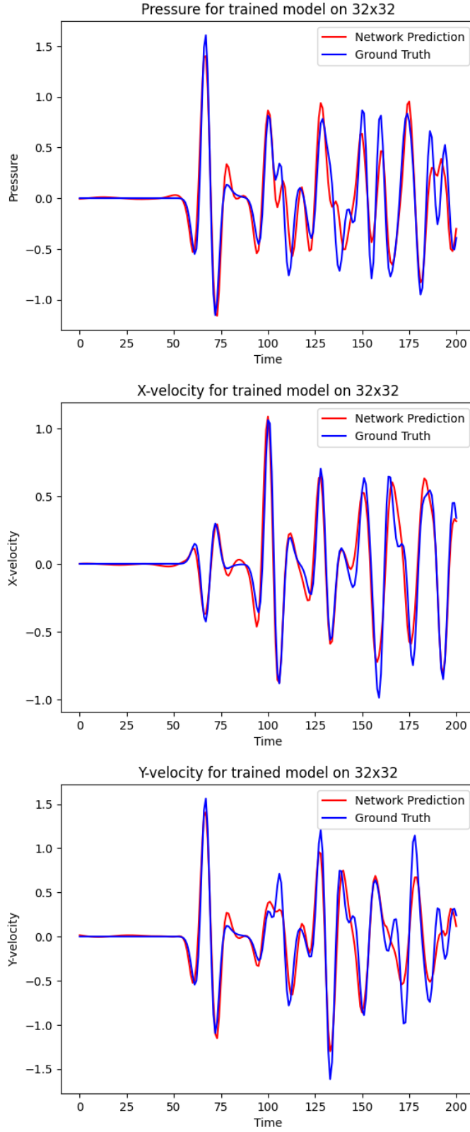
Figure 4.3: Results for pressure x and y-velocity for trained model on 32 \times 32 grid
