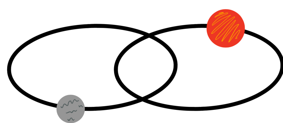
Fig. 2: Two Body Problem
