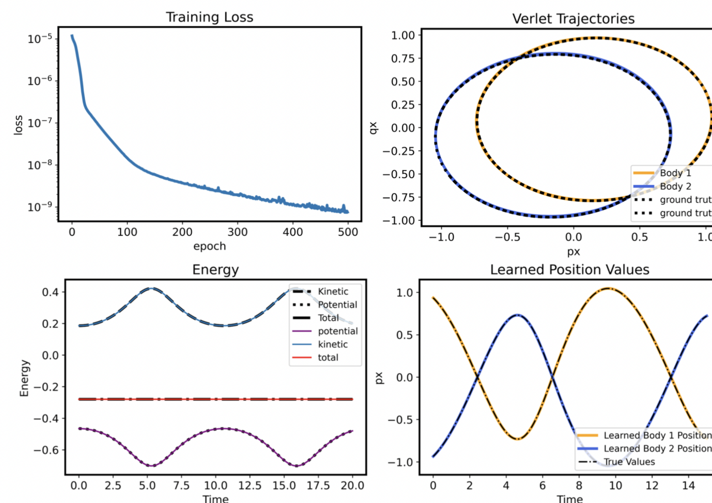
Fig. 4: Two Body Problem
