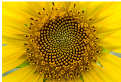
Figure 1: Spirals in a sunflower (Source).
