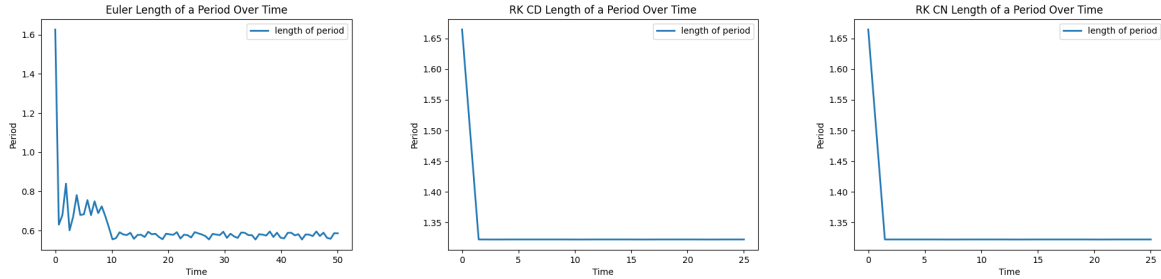
Figure 10: Convergence to a period for each scheme over time. Euler: 0.56-0.58; RK4 CD: 1.32; RK4 CN: 1.32
